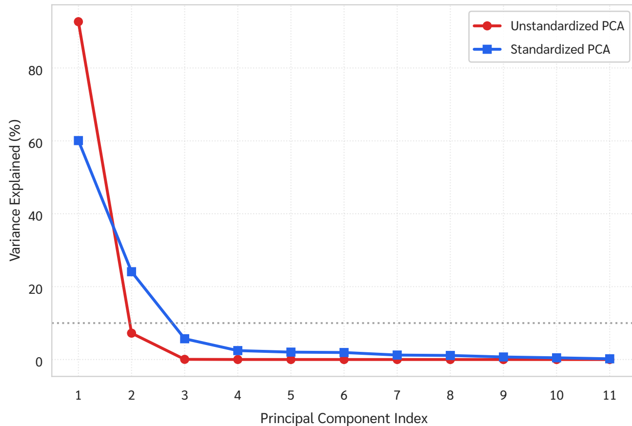
(A) Scree Plot: Proportion of Variance Explained (PVE)
