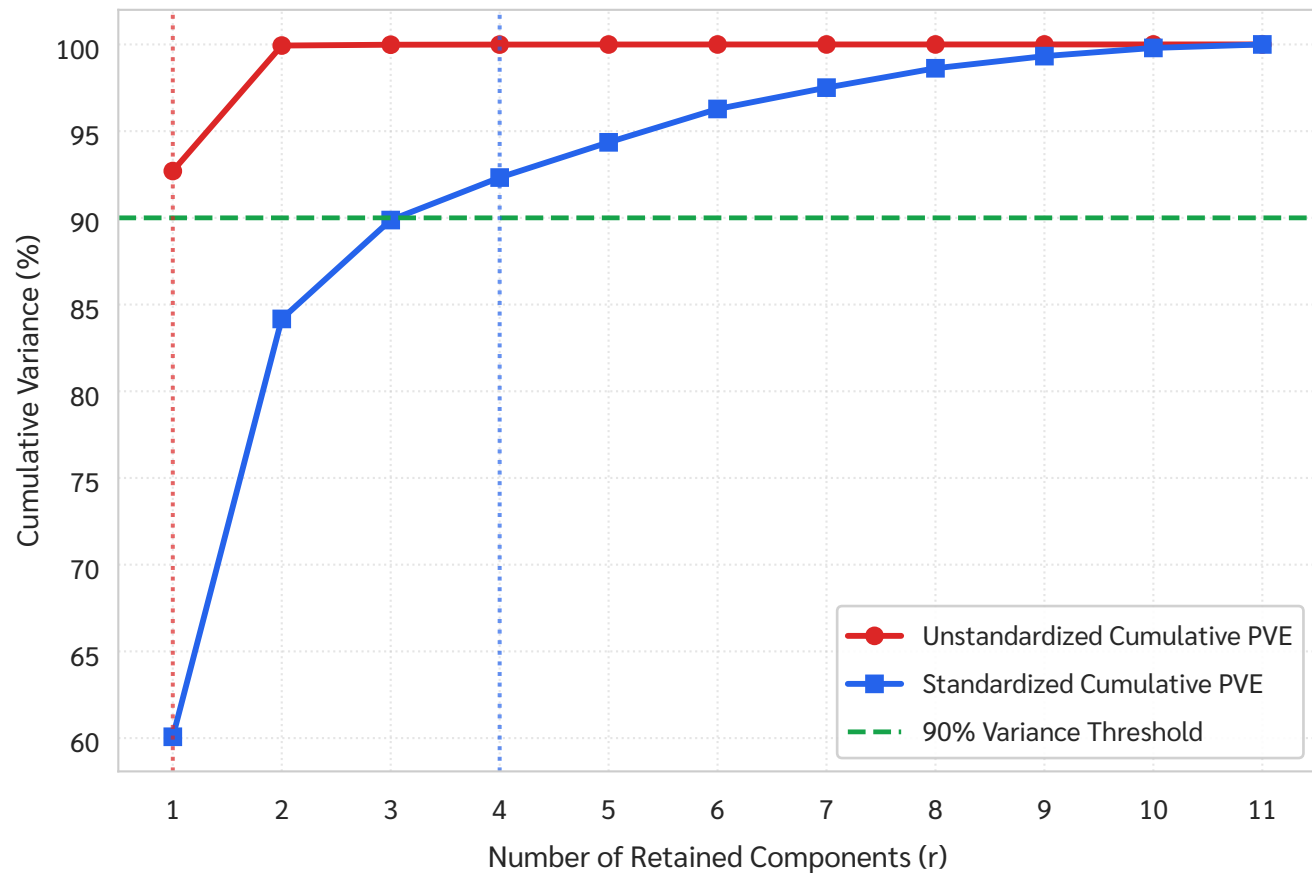
(B) Cumulative Variance Explained vs. 90% Threshold
